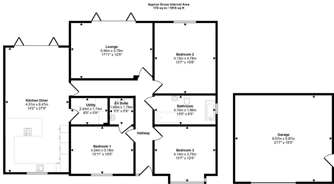
Floorplan Approx 139 sq m / 1500 sq ft
